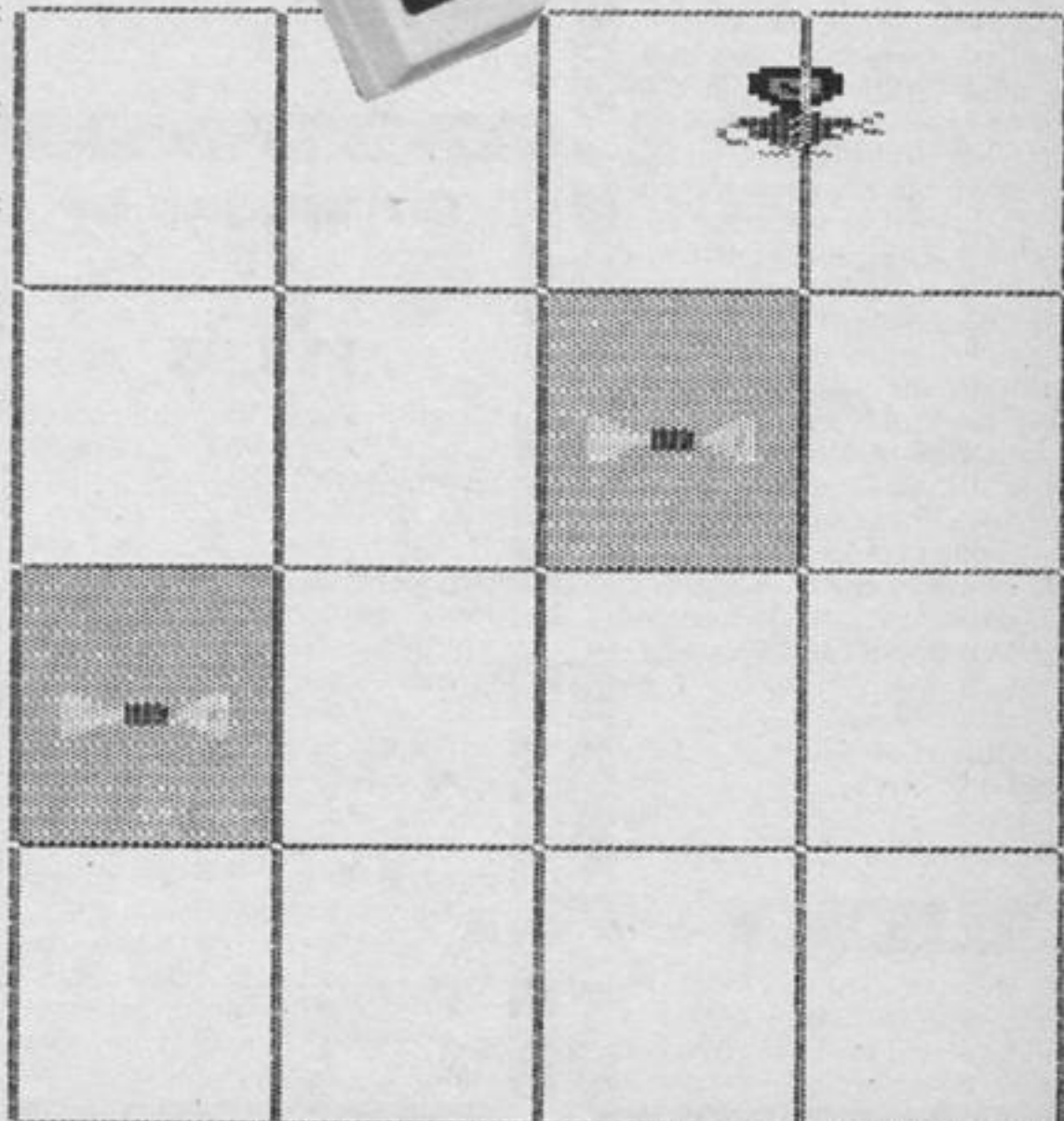
Screen dump
